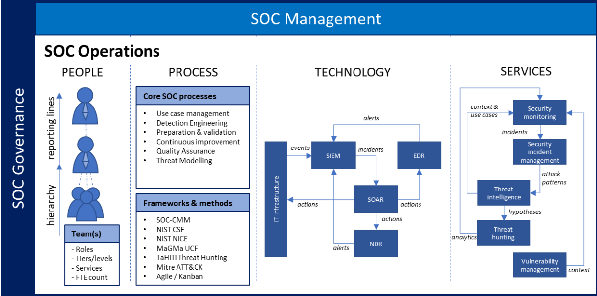
Figure 2: SOCTOM example visualisation
